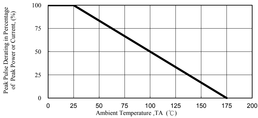
Fig. 1 - Pulse Derating Curve
